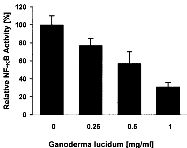
Figure 6. Ganoderma lucidum inhibits NF-κB in PC-3 cells. PC-3 cells were transfected with 1 μg NF-κB-CAT reporter construct and 3 μg β-galactosidase expression vector pCHI10. Twenty-four hours after transfection, the cells were treated with Ganoderma lucidum , and NF-κB was measured as described under Materials and methods. The results are expressed as the percentage of relative NF-κB activity. Each bar represents the mean ± SD of three experiments.
